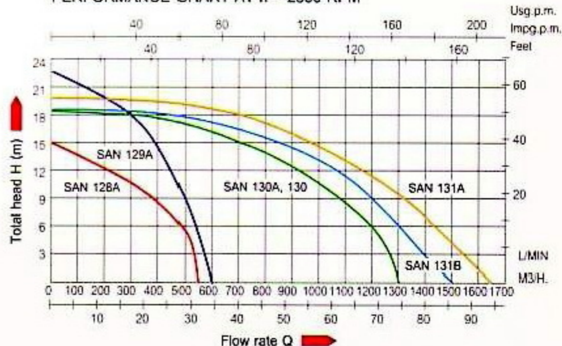
PERFORMANCE CHART AT n = 2850 RPM
